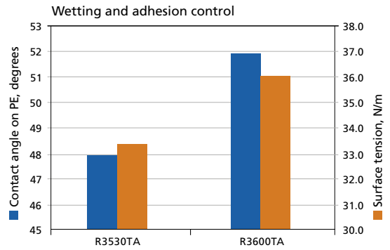
The surface tension and contact angle on PE of the acrylates of trifunctional polyols R3530 and R3600
