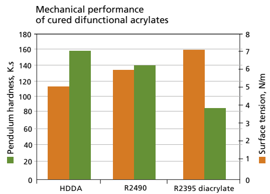
Highest flexibility with R2395DA compared to alternative difunctional monomers
