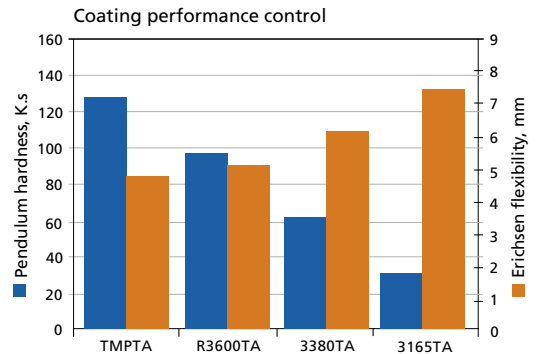
The hardness and flexibility of the acrylates of trifunctional polyols TMP, R3600, 3380 and 3165
